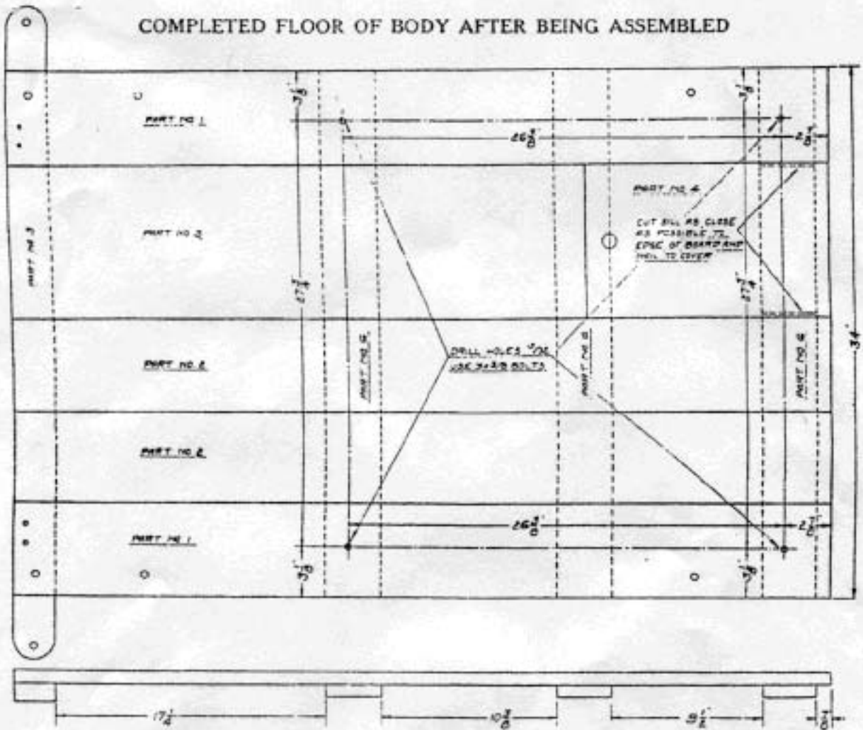
DRAWINGS 1-2-3-4—DETAIL OF FLOOR BOARDS
