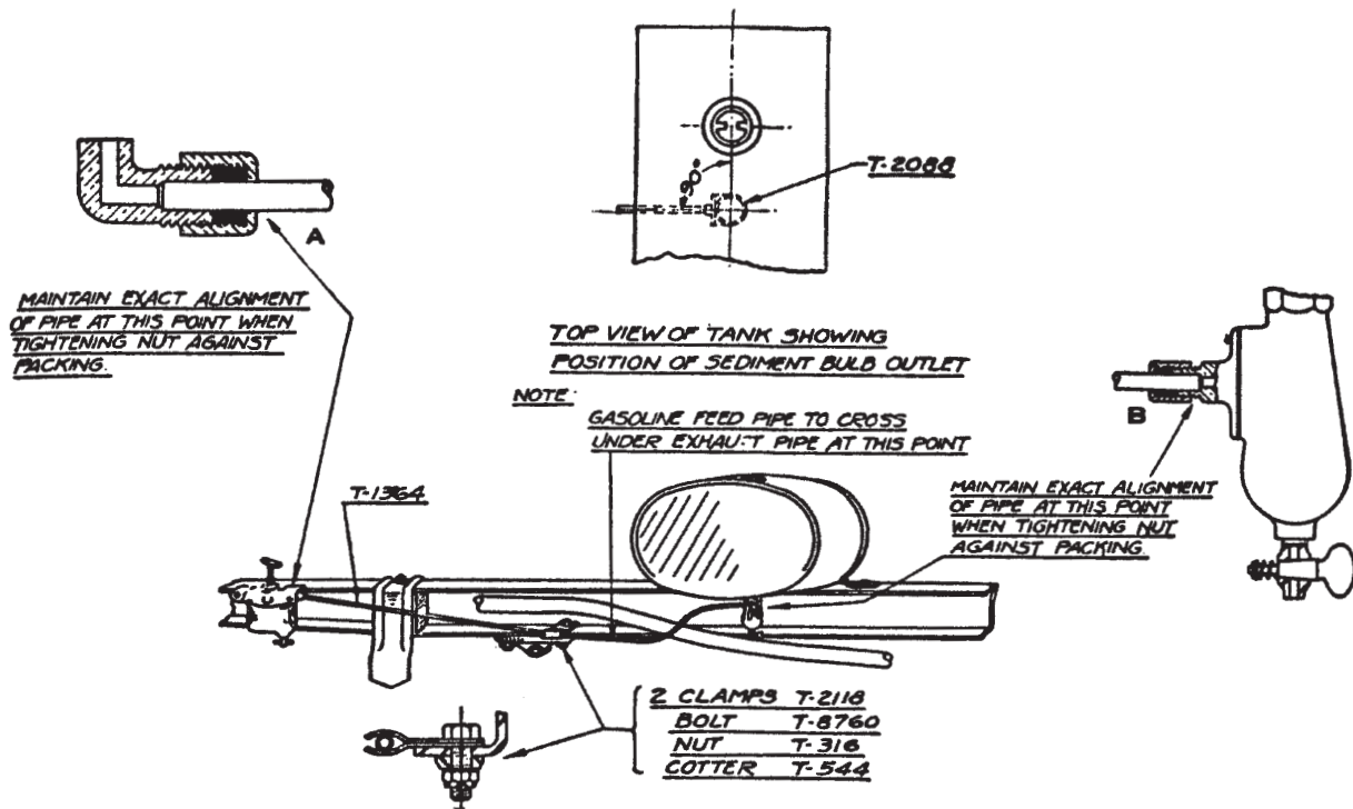
Method of Assembling Gasoline Feed Pipe on Touring, Roadster, Coupe-1924, 4 Door Sedan & Model-TT
